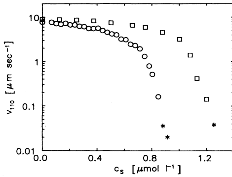
FIG. 6. The measured interfacial velocities v_{110} as a function of salt concentration, the circles are data on the A particles at the fixed volume fraction \Phi_A=0.003 and the squares are data on the B particles at \Phi_B=0.0022 . In both curves the stars denote points measured in the coexistence region.
