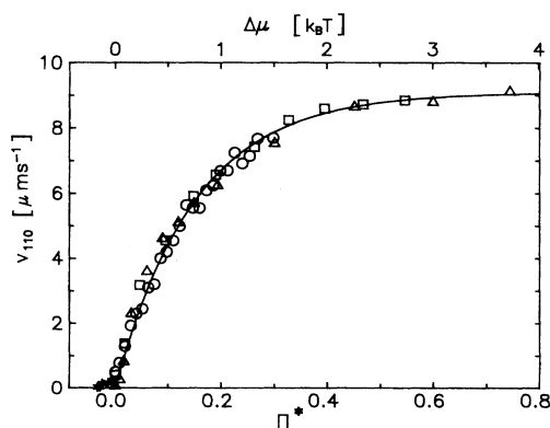
FIG. 8. The growth velocity v_{110} plotted versus the reduced density difference \Pi^* for all three experimental series (symbols as in Figs. 5 and 6). Within the experimental error all data points coincide on one master curve. A Wilson-Frenkel law [Eq. (1)] is fitted to the data with positive \Pi^* and shown as solid line. The best fit parameters are v_\infty = 9.1 \pm 0.1 \mu\text{m s}^{-1} and B = 6.7 \pm 0.1 k_B T . The chemical potential difference \Delta\mu between solid and melt used in the upper x axis was derived from \Pi^* using the conversion factor B .
