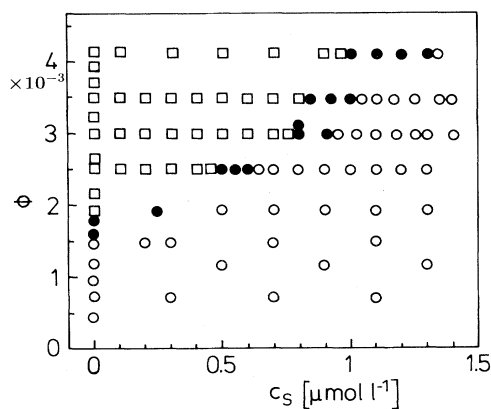
FIG. 1. The experimental phase diagram of the A particles in dependence on the salt concentration c and the volume fraction \Phi . Squares denote the bcc phase and open circles the fluid phase. The two phases are divided by a coexistent region denoted by closed circles.
