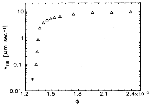
FIG. 7. The measured interfacial velocities v_{110} as a function of the volume fraction \Phi_B of B particles at no added salt. The stars again denote points measured in the coexistence region.
