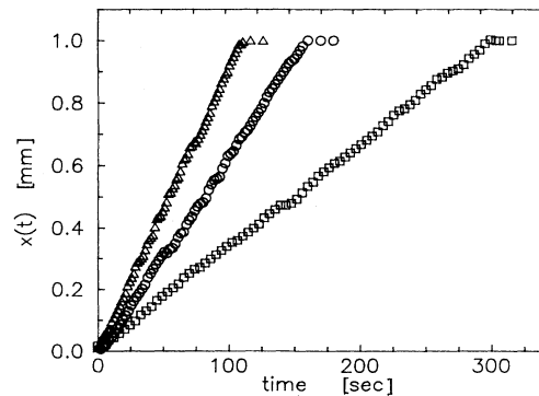
FIG. 5. Thickness x(t) of the crystalline phase plotted as a function of time for different suspension parameters. The triangles are B particles at \Phi = 0.0019 and c = 0 ; the circles are A particles at \Phi = 0.003 and c = 0.27 \mu\text{mol l}^{-1} , and the squares are B particles at \Phi = 0.0022 and c = 1.08 \mu\text{mol l}^{-1} .
